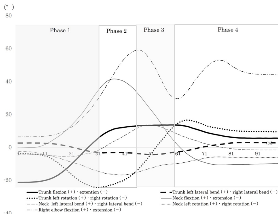
Fig.4 Transition of average joint angle at 60^\circ shoulder abduction
